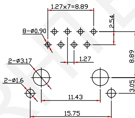
PCB Layout
